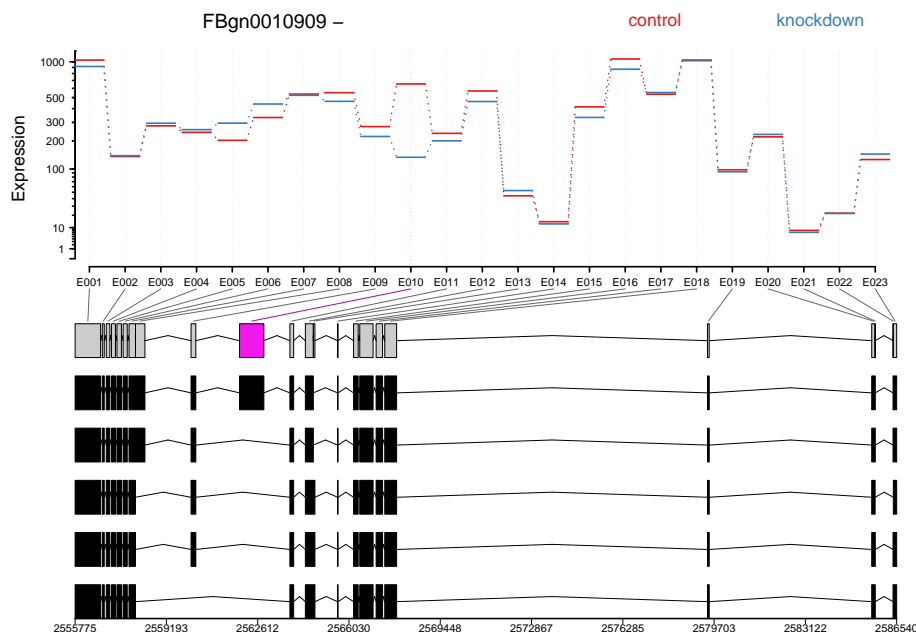
Figure 4: Transcripts
