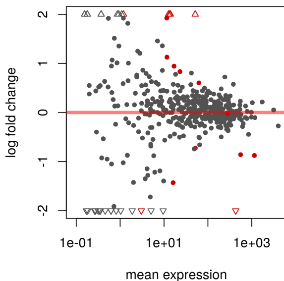
Figure 2: MA plot
