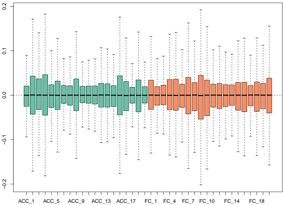
Figure 3: Heatmap and RLE Heatmap (upper panel): colors in heatmap highlight the distance matrix, obtained by Spearman’s correlation metric: color gradient ranges from dark green , meaning ‘minimum distance’ ( i.e. dissimilarity = 0, correlation = 1), to light green green . On the top of heatmap, horizontal bars represent class and covariates. Each variable is differently colored (see legend). On the top and on the left side of the heatmap the dendrograms are drawn. Clusters can be easily identified. RLE (lower panel): a boxplot of the distribution of expression values computed as the difference between the expression of each gene and the median expression of that gene across all samples. Here, since all medians are very close to zero, it appears that all the samples are well-normalized and do not present any quality problems.
